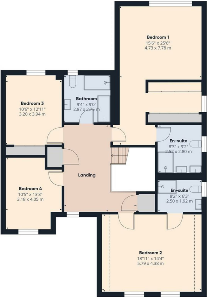
First Floor Main House
